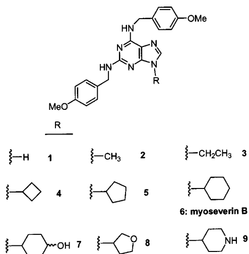
Figure 4. Structure of myoseverin derivatives.
